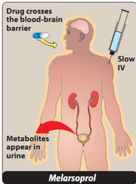
Figure 36.14 Administration and fate of melarsoprol .
