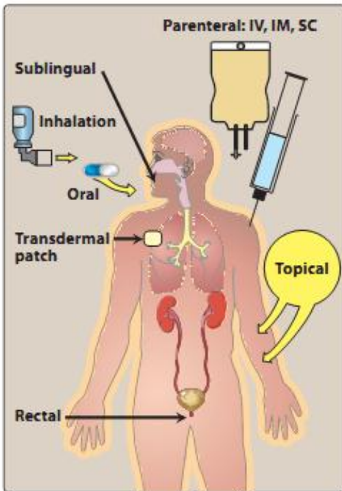
Figure 1.2 Commonly used routes of drug administration. IV = intravenous; IM = intramuscular; SC = subcutaneous.
