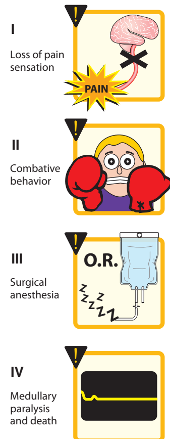
Figure 11.3 Stages of anesthesia. O.R. = operating room.
