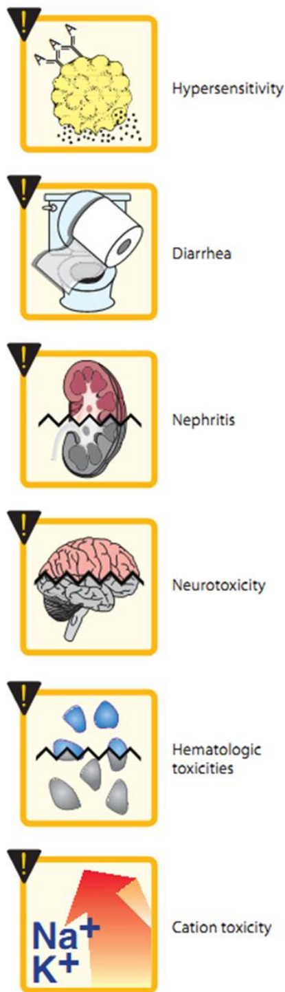
Figure 31.9 Summary of the adverse effects of penicillin.
