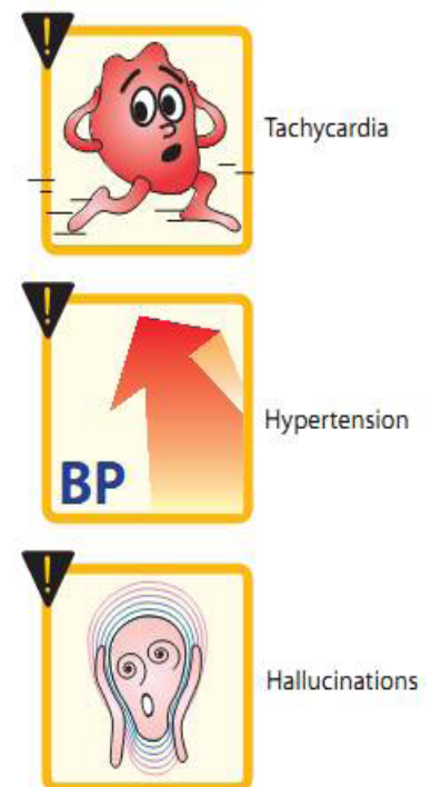
Figure 10.12 Adverse effects of tetrahydrocannabinol .
