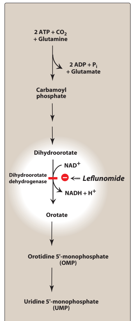
Figure 41.17 Site of action of leflunomide .
