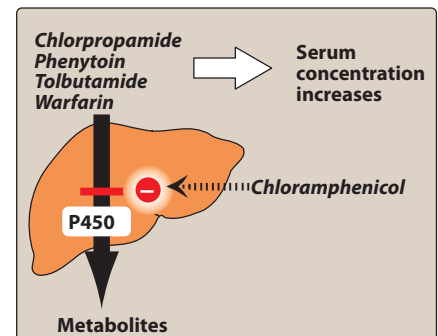
Figure 32.19 Inhibition of the cytochrome P450 system by chloramphenicol .
