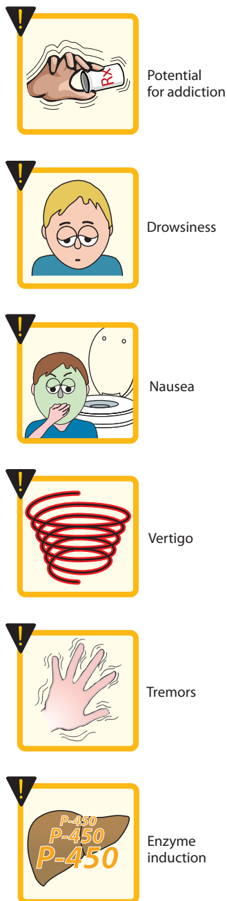
Figure 9.9 Adverse effect of barbiturates.
