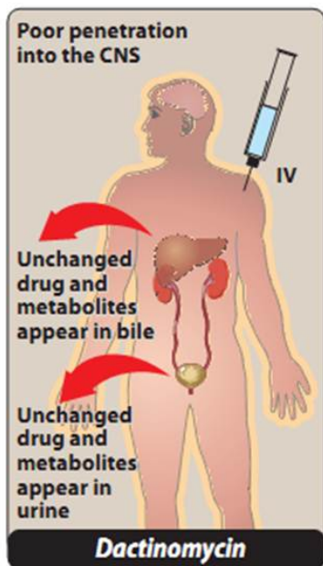
Figure 39.17 Administration and fate of dactinomycin . CNS = central nervous system; IV = intravenous.
