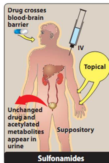
Figure 33.10 Administration and fate of the sulfonamides.
