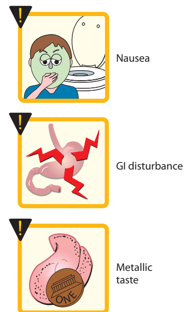
Figure 36.4 Adverse effects of metronidazole .
