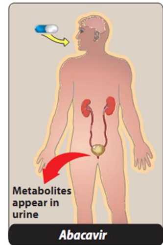
Figure 38.21 Administration and fate of the abacavir .
