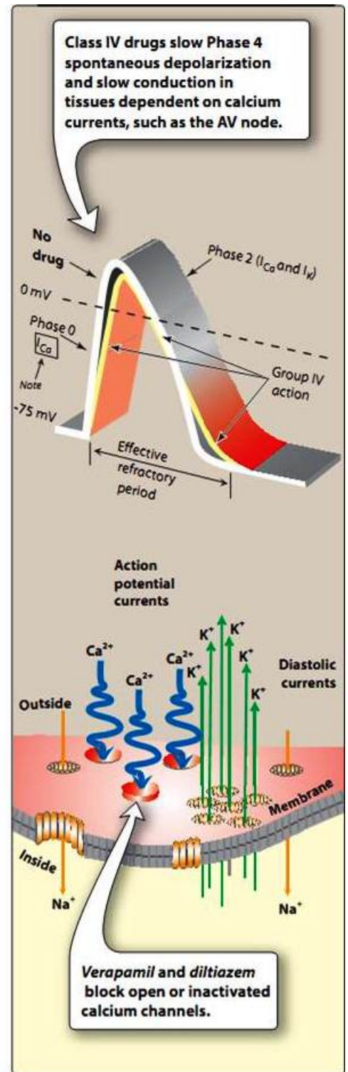
Figure 17.10 Schematic diagram of the effects of Class IV agents. I_{Ca} and I_K are transmembrane currents due to the movement of Ca^{2+} and K^+ , respectively.
