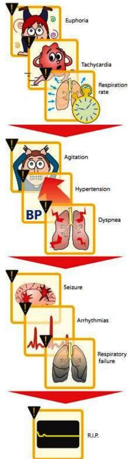
Figure 10.8 Major effects of cocaine use.
