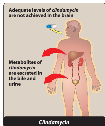
Figure 32.20 Administration and fate of clindamycin .
