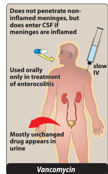
Figure 31.17 Administration and fate of vancomycin .
