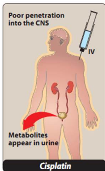
Figure 39.31 Administration and fate of cisplatin . CNS = central nervous system; IV = intravenous.
