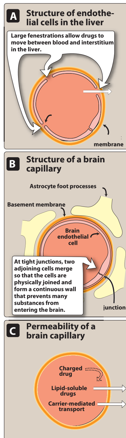
Figure 1.13 Cross section of liver and brain capillaries.
