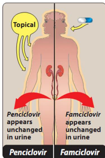
Figure 38.14 Administration and metabolism of penciclovir and famciclovir .
