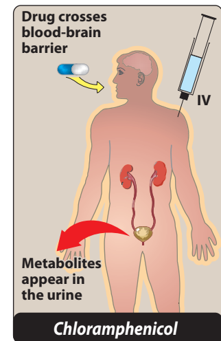
Figure 32.18 Administration and fate of chloramphenicol .
