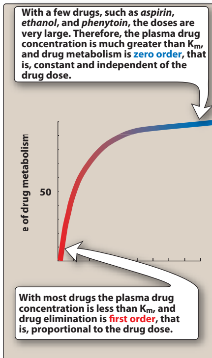
Figure 1.16 Effect of drug dose on the rate of metabolism.
