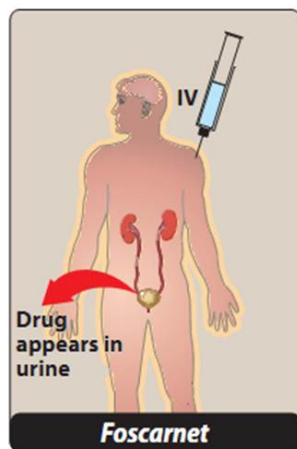
Figure 38.12 Administration and metabolism of foscarnet .
