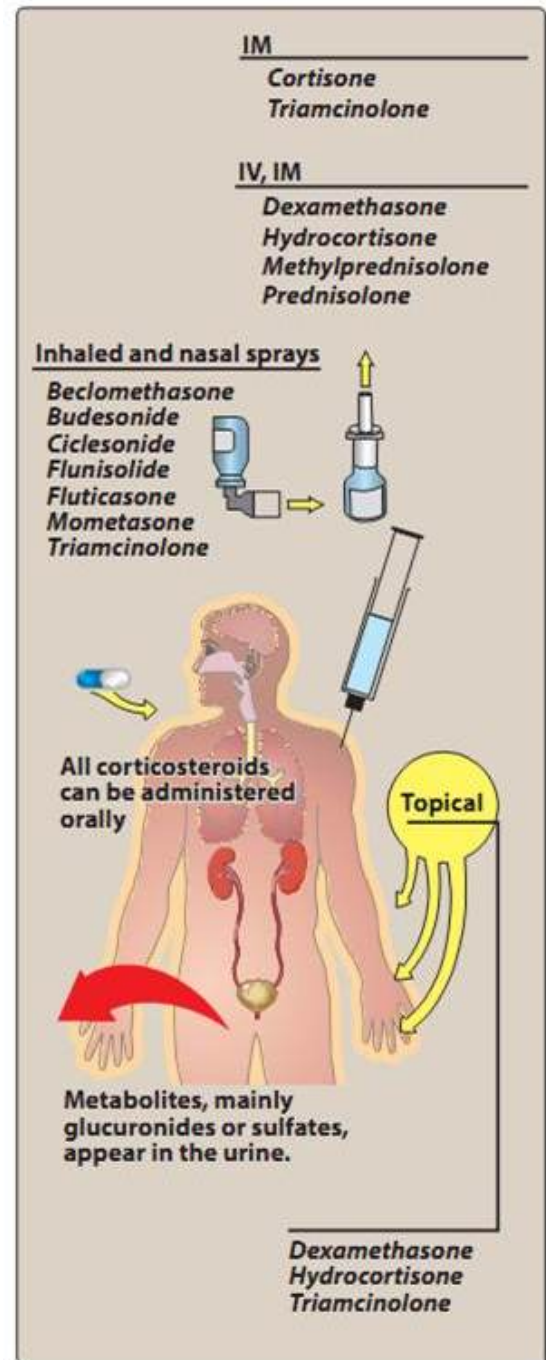
Figure 26.5 Routes of administration and elimination of corticosteroids.
