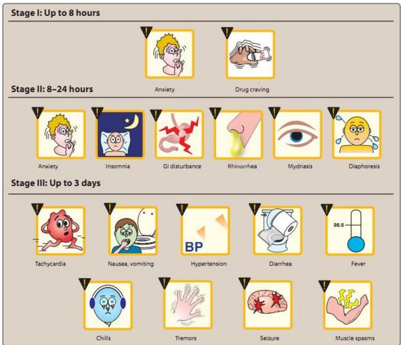
Figure 14.13 Opiate withdrawal syndrome. GI = gastrointestinal.
