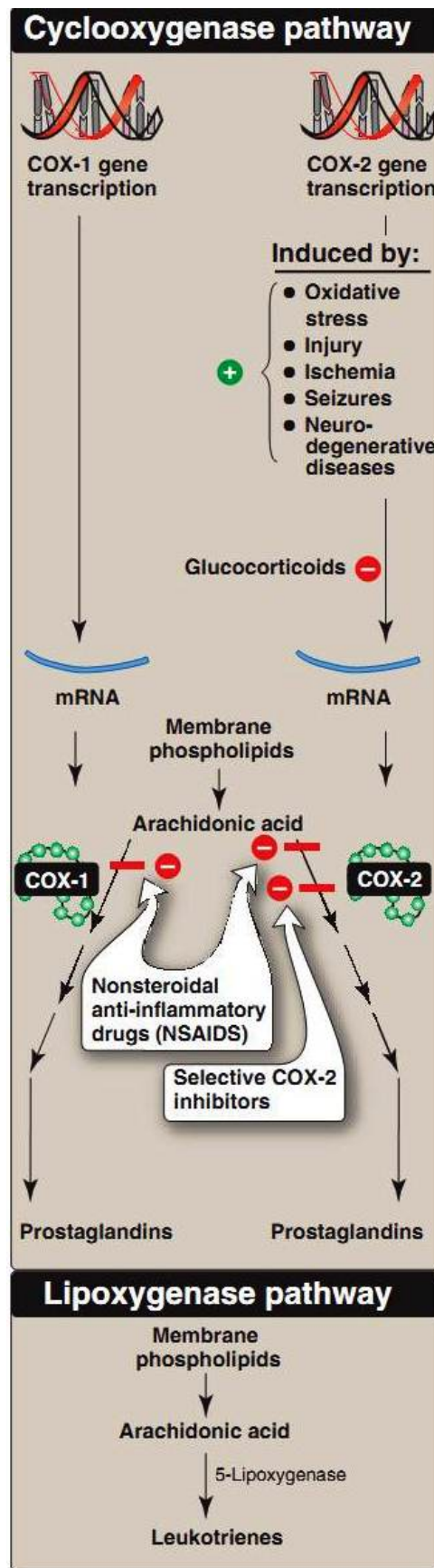
Figure 41.3 Synthesis of prostaglandins and leukotrienes. COX = cyclooxygenase.
