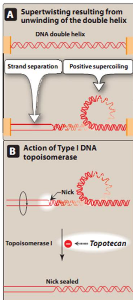
Figure 39.32 Action of Type I DNA topoisomerases.
