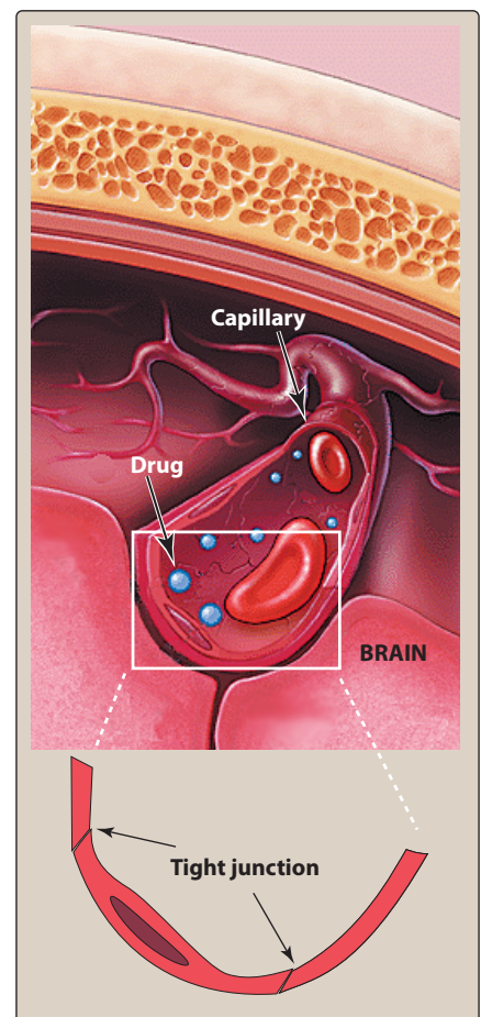
Figure 30.4 Essential features of the blood-brain barrier.
