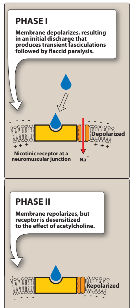
Figure 5.12 Mechanism of action of depolarizing neuromuscular-blocking drugs.
