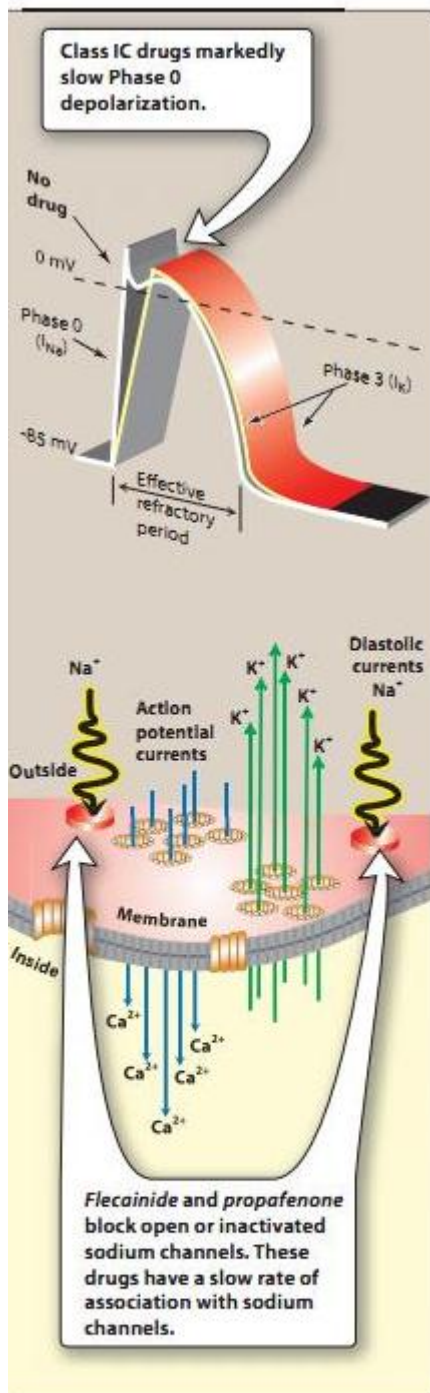
Figure 17.7 Schematic diagram of the effects of Class IC agents. I_{Na} and I_K are transmembrane currents due to the movement of Na^+ and K^+ , respectively.
