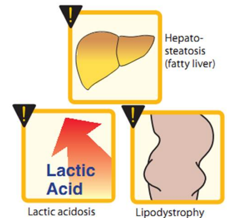
Figure 38.23 Some adverse reactions of nucleoside analogs.
