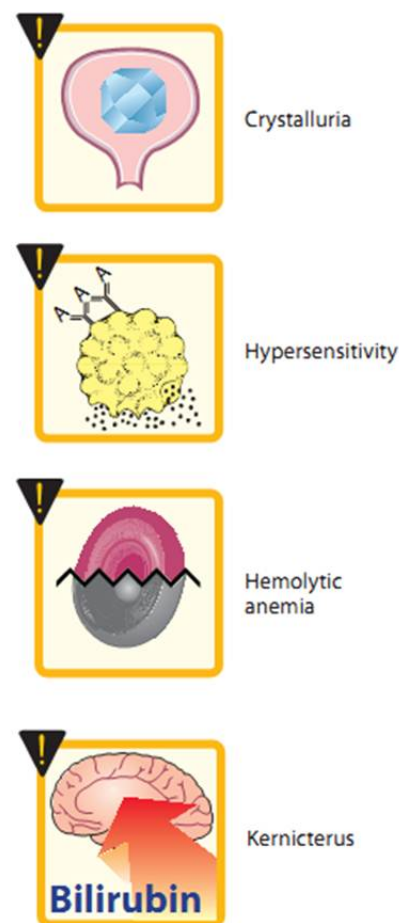
Figure 33.11 Some adverse reactions to sulfonamides.
