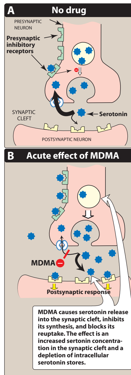
Figure 43.9 Proposed mechanism of action of methylenedioxymethamphetamine (MDMA).
