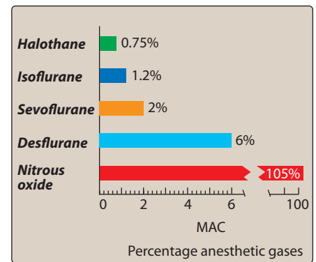
Figure 11.4 Minimal alveolar concentrations (MAC) for anesthetic gases.
