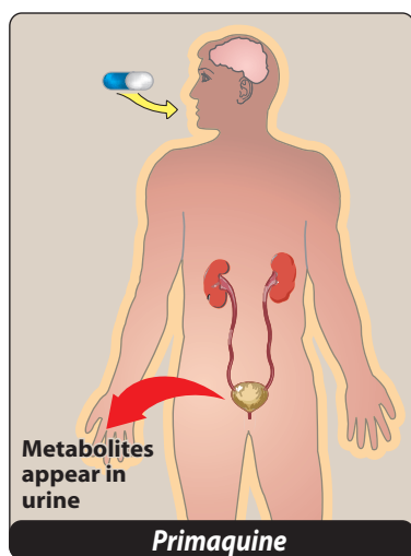
Figure 36.7 Administration and fate of primaquine .
