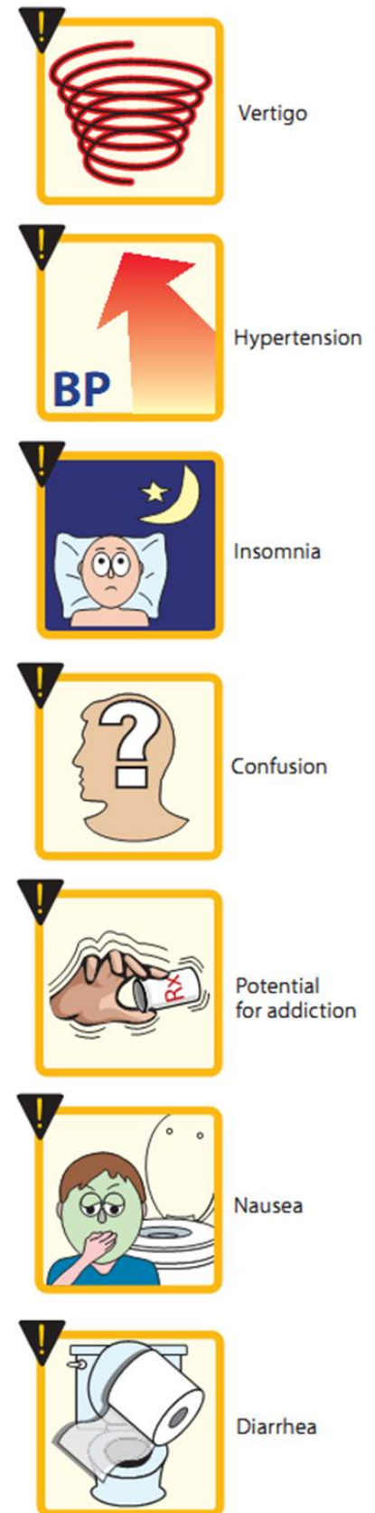
Figure 10.10 Adverse effects of amphetamines.
