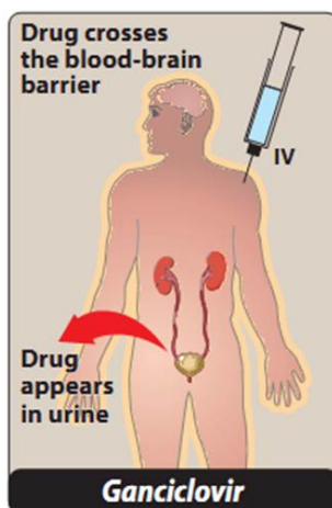
Figure 38.13 Administration and metabolism of ganciclovir .
