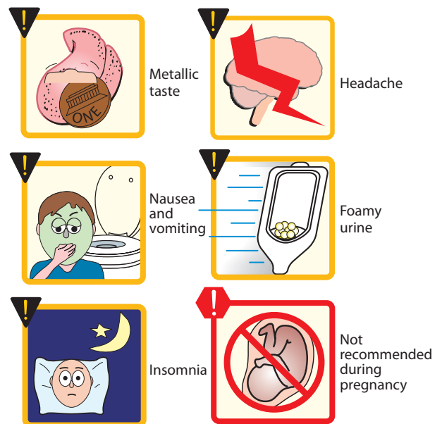
Figure 31.21 Some cautions and adverse effects of telavancin .
