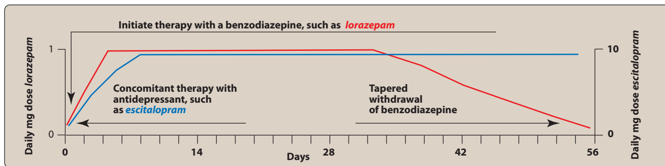
Figure 9.6 Treatment guideline for persistent anxiety.
