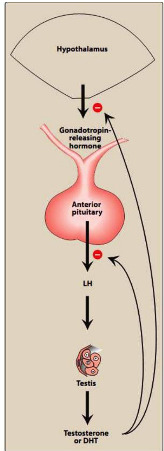
Figure 25.11 Regulation of secretion of testosterone. DHT = 5- \alpha -dihydrotestosterone; LH = luteinizing hormone.
