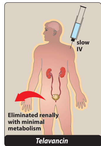
Figure 31.20 Administration and fate of telavancin .
