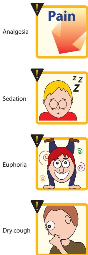
Figure 14.10 Some actions of codeine .
