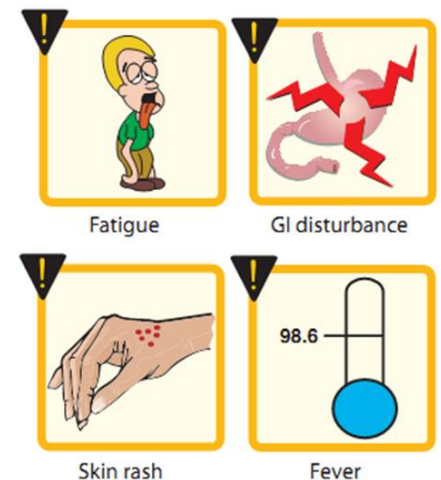
Figure 38.22 Hypersensitivity reactions to abacavir .
