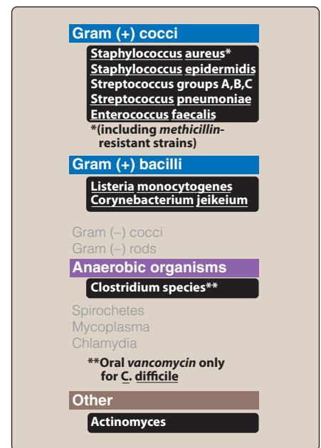
Figure 31.16 Antimicrobial spectrum of vancomycin .
